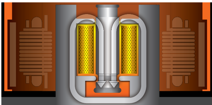
Hydraulic-Bearing Technology
